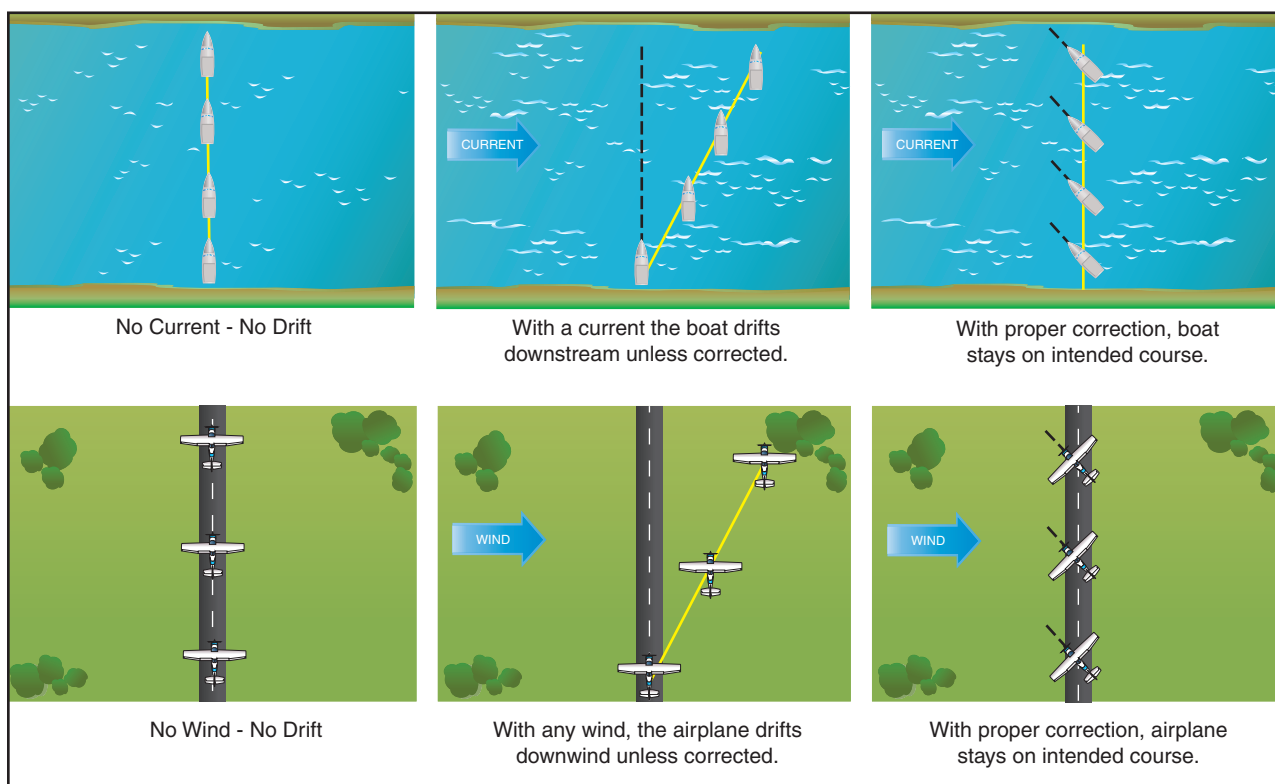
Figure 6-1. Wind drift.
