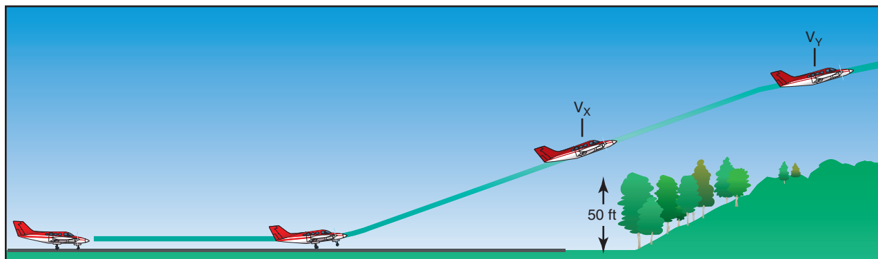
Figure 12-9. Short-field takeoff and climb.
