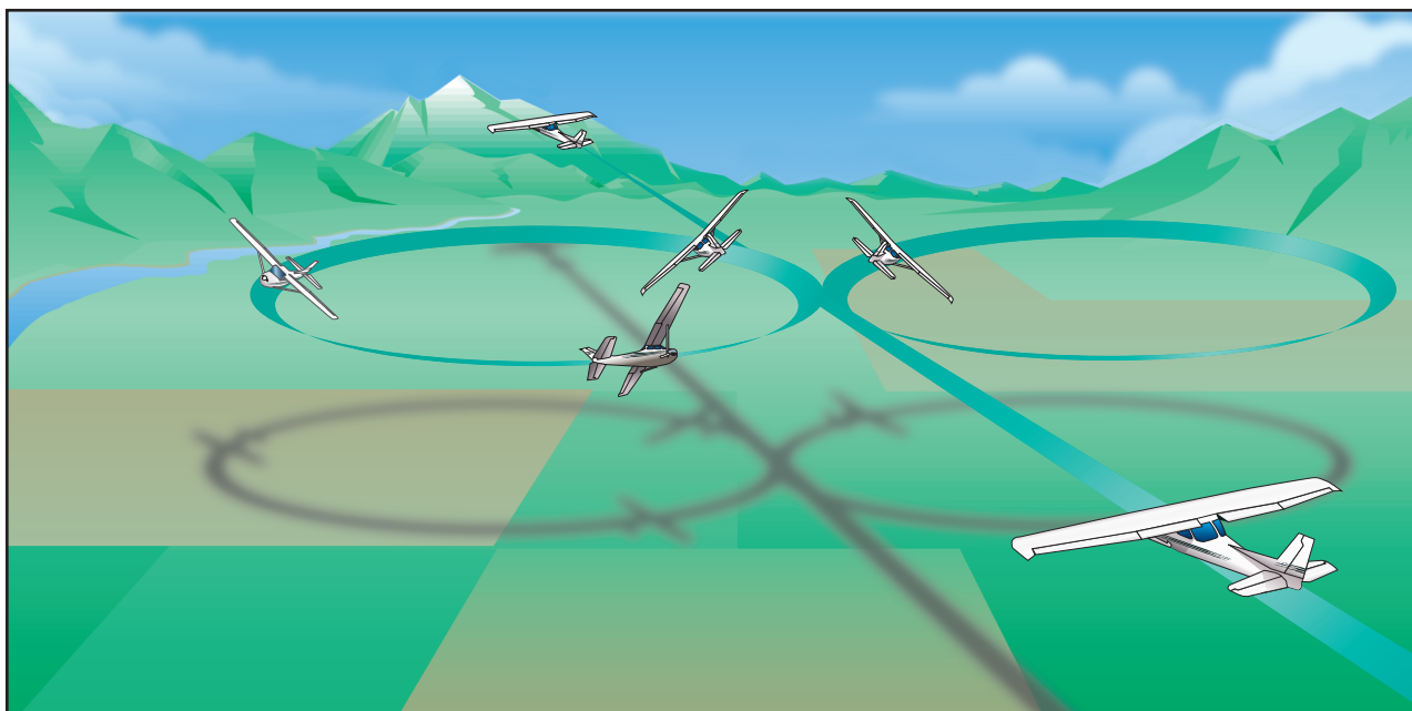
Figure 9-1. Steep turns.
