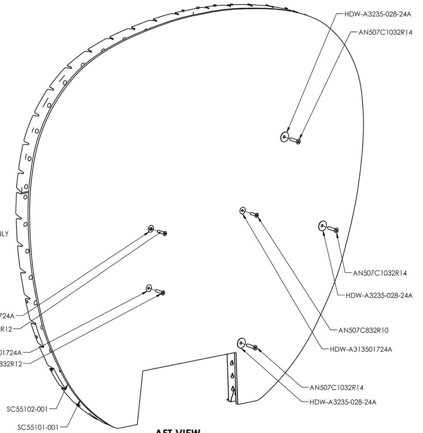
AFT VIEW
