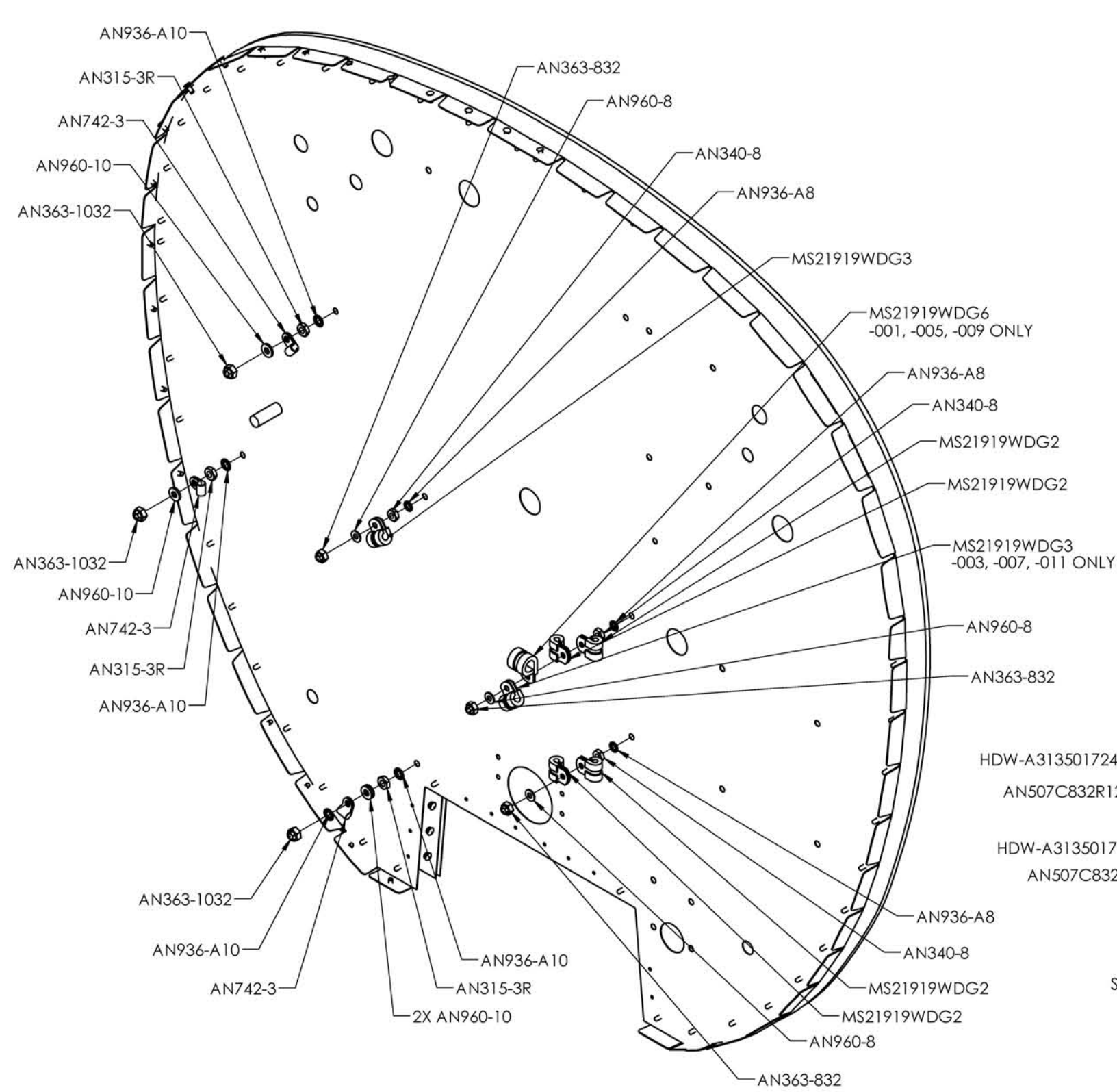
FRONT VIEW
